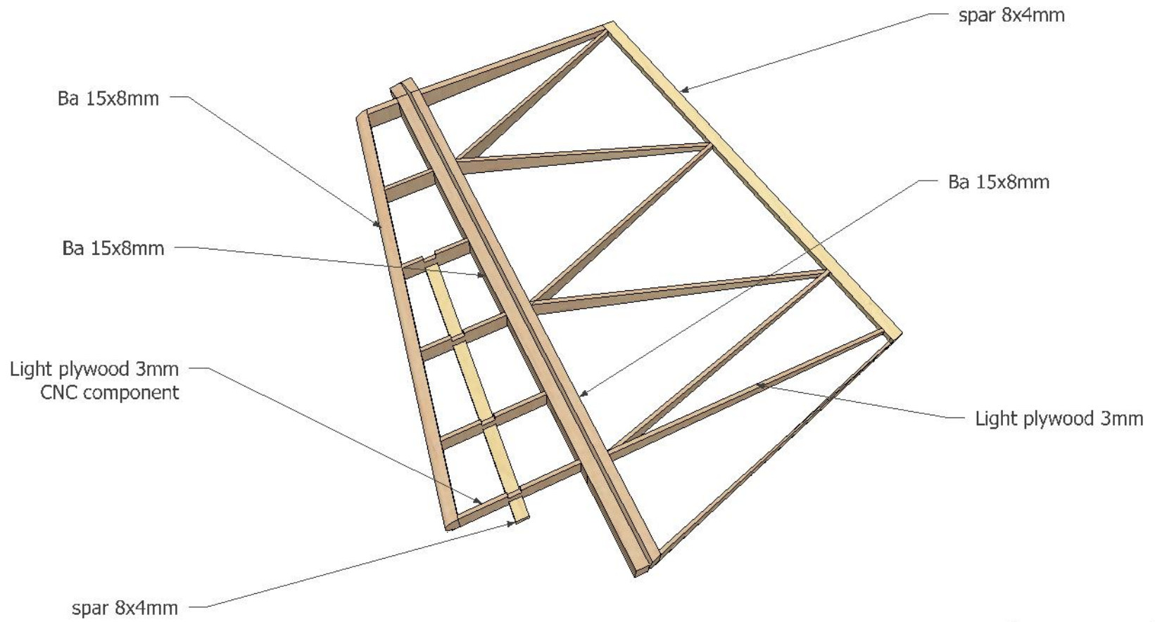
Grune Post - Rudder
